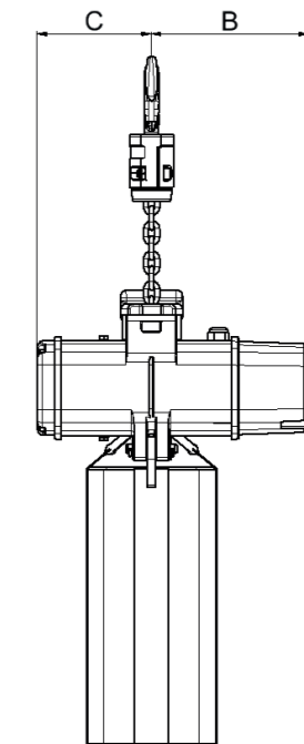
Chain Hoist with suspension eye
