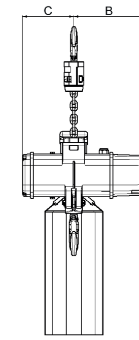
Chain Hoist with hook suspension
